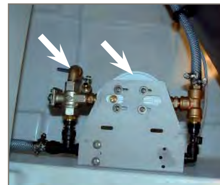
VALVES FOR SELECTION AND WATERMAKER FILTER
