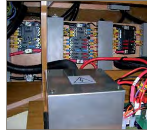
AUTOMATIC BREAKERS BEHIND THE ELECTRICAL PANEL
