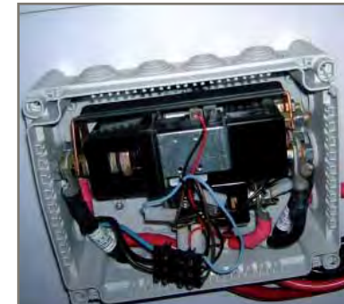
COUPLING RELAY
