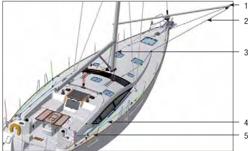
SYMMETRIC SPINNAKER SYSTEM
