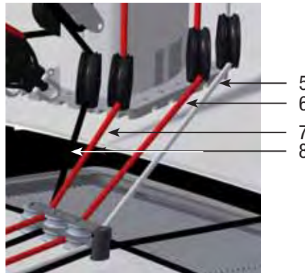
STARBOARD MAST FOOT
